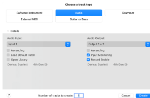
Logic Pro
